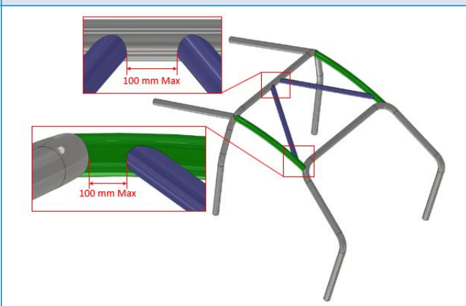
Dessin/Drawing SC-10b
