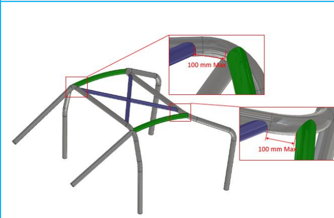
Dessin/Drawing SC-9a
