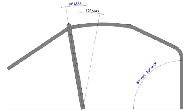
Dessin/Drawing SC-5
