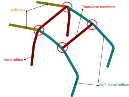
Dessin/Drawing SC-4
