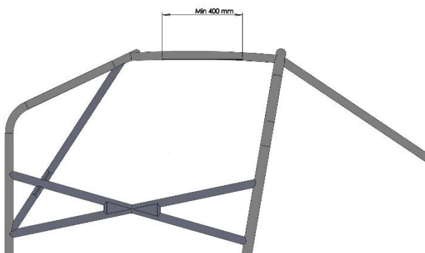
Dessin/Drawing SC-CC-3
