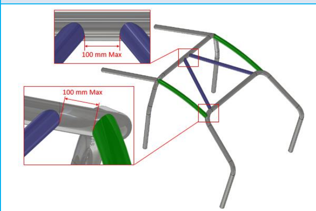
Dessin/Drawing SC-10a
