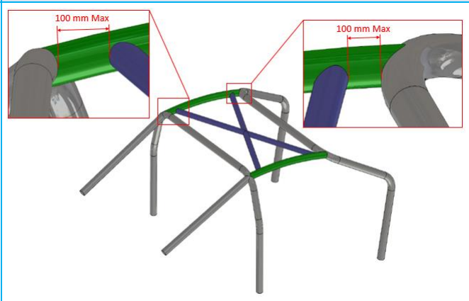
Dessin/Drawing SC-9b
