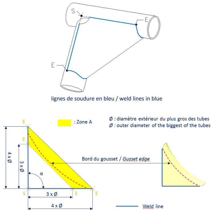
Dessin/Drawing SC-GU-1
