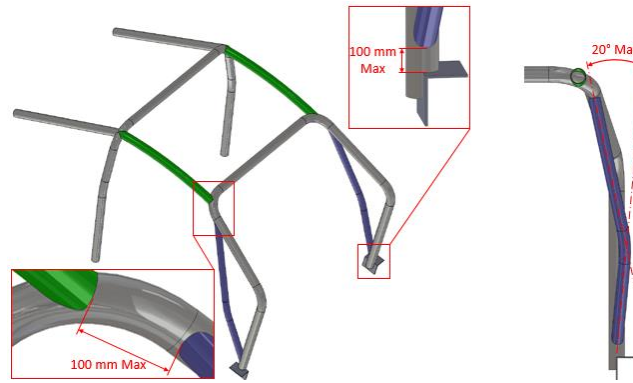
Dessin/Drawing SC-12
