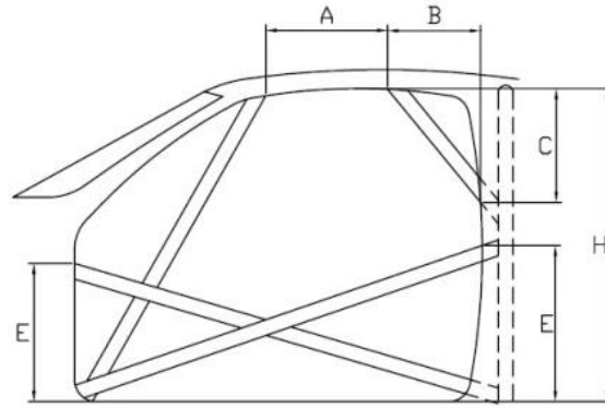
Dessin/Drawing SC-15
